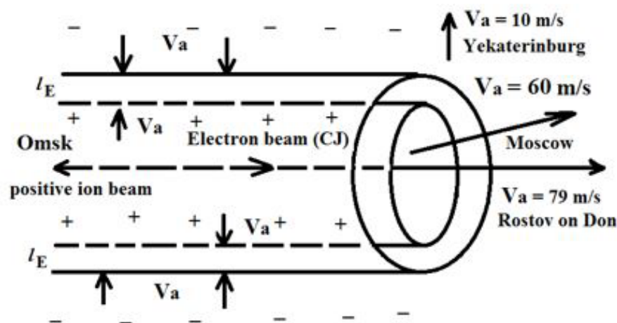
Figure 7: 3D schemes: formation of the Vysikaylo’s laser-gun by ambipolar drifts directed towards the boundaries of the plasma system and the propagation of plasma disturbances in the ionosphere at the speed of ambipolar drift V_a (these are analogs of Mach’s shock waves) of plasma disturbances after the destruction of the meteoroid according to the Vysikaylo’s fragmentation scheme.
