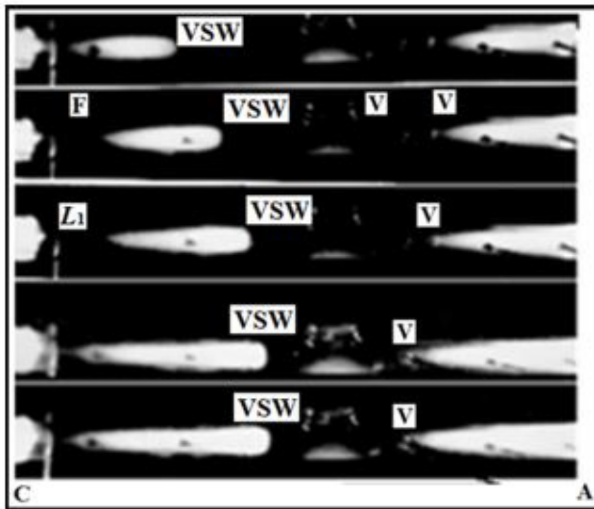
Figure 5: Photo of energy cumulation due to dynamic surface tension in plasmoids:
