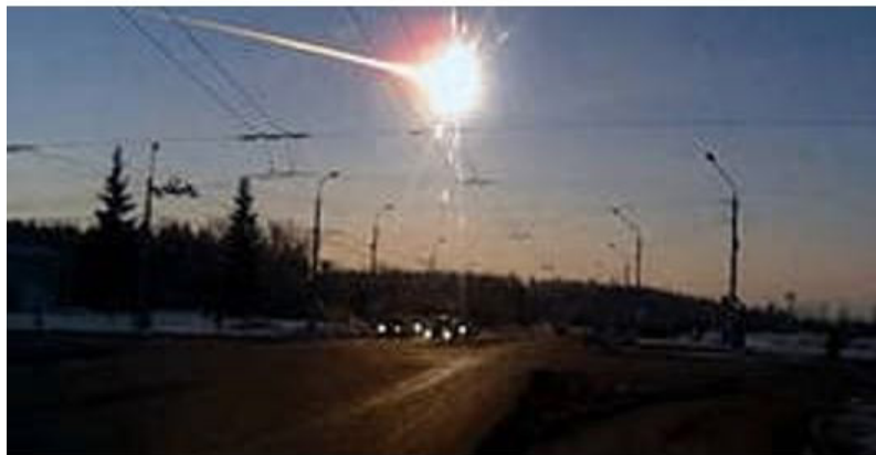
Figure 1: Photographic evidence of plasma cumulation in a asteroid wake. This is a photograph (Marat Akhmetvaleev, 2013) of the Coulomb explosion (see [8] for more details).
