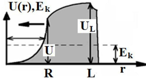
Figure 3: This is a potential barrier U(r) for electrons in a cylindrical plasmoid with a positive charge. The characteristic transverse size of the potential well in this case is greater than the radius of the system and is determined by its length ( \approx L ), and not by the radius ( R ).
